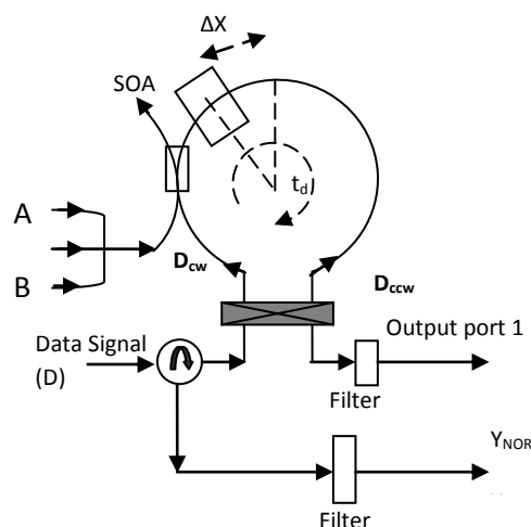
Fig1. TOAD based 3- input NOR gate
